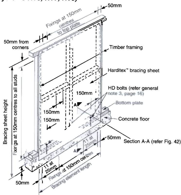
Fig. 41 HARDITEX™ GROUP NAIL FIXING FOR CONCRETE FLOORS (Systems HT6, HT7, HT8)
