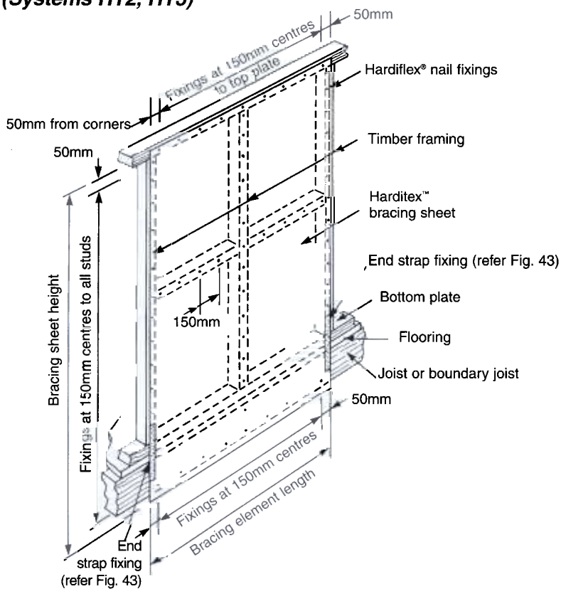
Fig. 38 HARDITEX™ TO TIMBER JOISTS WITH END STRAPS (Systems HT2, HT3)
