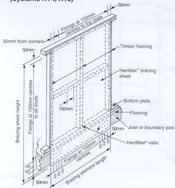
Fig. 40 HARDITEX™ GROUP NAIL FIXING TO TIMBER JOISTS (Systems HT4, HT5)
