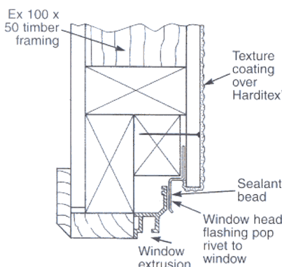
Fig. 62 JAMB DETAIL (ALTERNATIVE 2)
