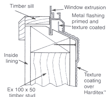
Fig. 60 SILL DETAIL (ALTERNATIVE 3)
