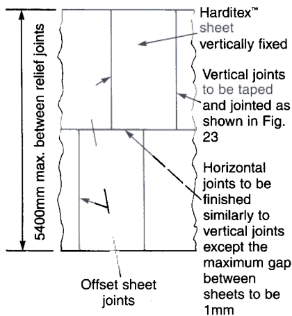
Fig. 12 OFFSET SHEET SET-OUT
