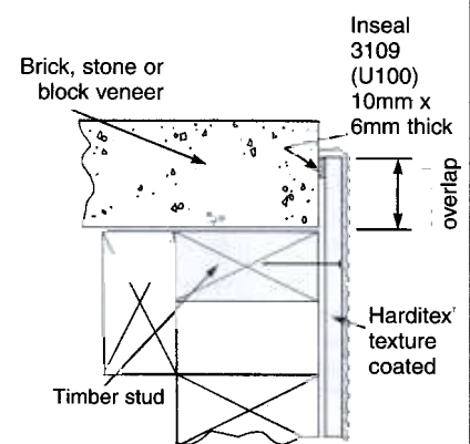
Fig. 66 BRICK VENEER TO HARDITEX™ EXTERNAL CORNER DETAIL
