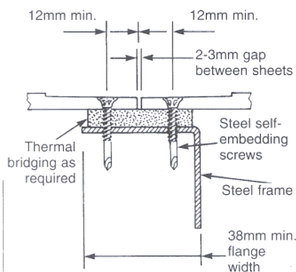
Fig. 30 FIXING TO NARROW STEEL FLANGES
