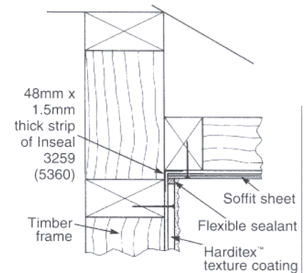
Fig. 64 HARDITEX™ TO SOFFIT DETAIL
