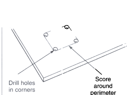
Fig. 9 RECTANGULAR HOLE FORMING
