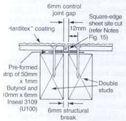
Fig. 21 VERTICAL BUTYNOL INSEAL CONTROL JOINT (ALTERNATIVE 1)
