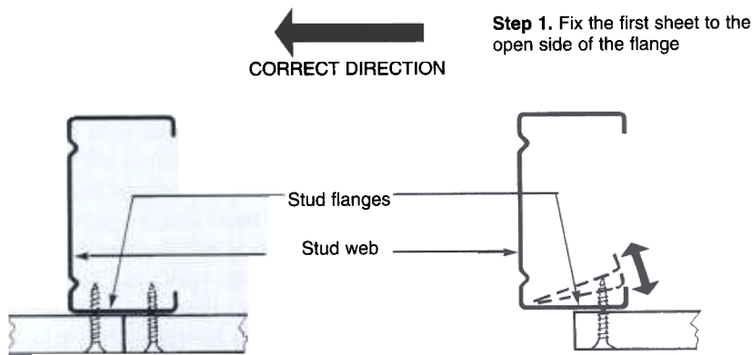
Fig. 33 CORRECT FIXING METHOD
