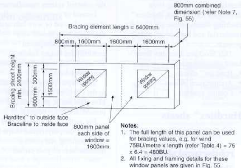
Fig. 56 HARDITEX™ / BRACELINE WINDOW OPENING PANEL – PANEL WITH TWO WINDOWS
