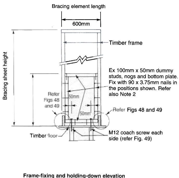
Fig. 46 600MM-WIDE HARDITEX™ TO TIMBER FLOOR (System HT10)
