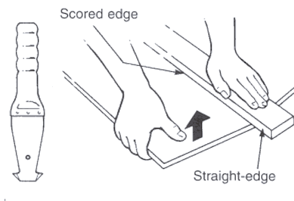
Fig. 3 SCORE-AND-SNAP METHOD
