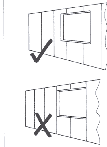
Fig. 10 SHEET LAYOUT FOR OPENINGS
