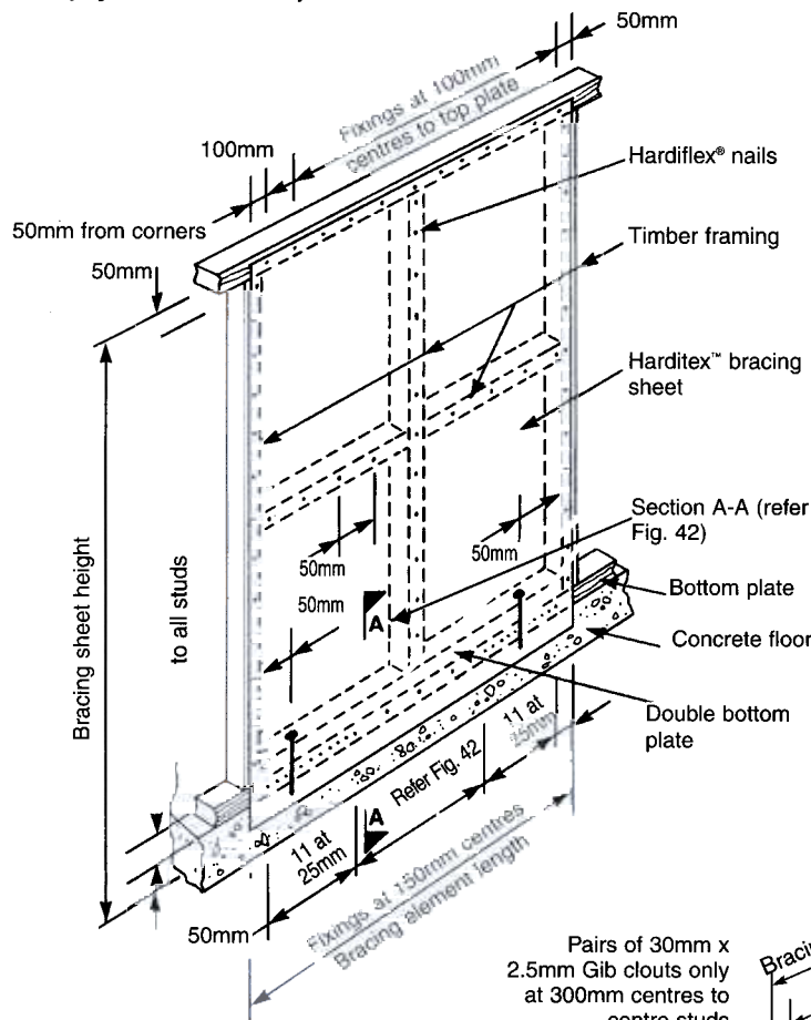
Fig. 52 HARDITEX™ / BRACELINE GROUP NAILING DETAIL ON CONCRETE FLOOR (System HT12B)
