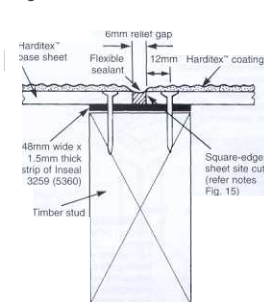
Fig. 16 VERTICAL SEALANT RELIEF JOINT (ALTERNATIVE 2)
