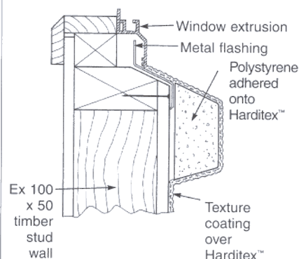
Fig. 60 SILL DETAIL (ALTERNATIVE 3)
