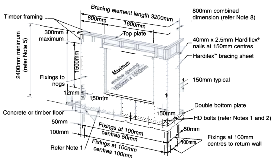
Fig. 55 HARDITEX™ / BRACELINE WINDOW OPENING PANEL
