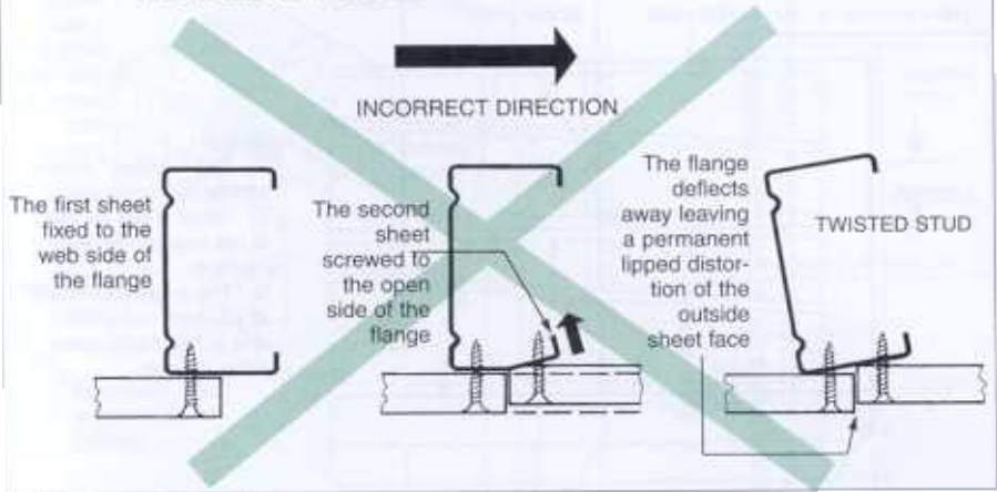
Fig. 34 INCORRECT FIXING RESULTING IN TWISTED FLANGE OR STUD
