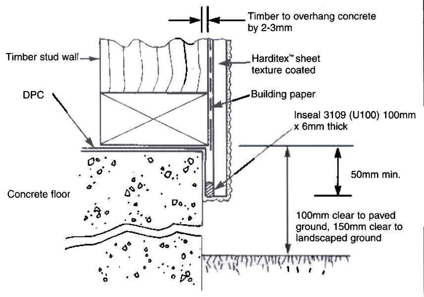
Fig. 14 HARDITEX™ OVERHANG DETAIL TO CONCRETE OR BLOCKWORK BASE
