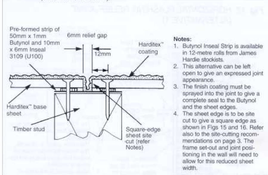
Fig. 15 VERTICAL BUTYNOL INSEAL RELIEF JOINT (ALTERNATIVE 1)
