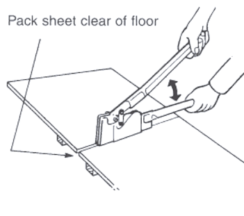
Fig. 4 HAND GUILLOTINE METHOD
