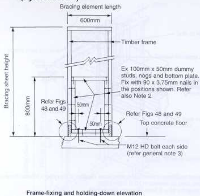
Fig. 45 600MM-WIDE HARDITEX™ TO CONCRETE FLOOR (System HT10)
