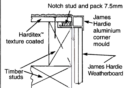
Fig. 65 CORNER DETAIL JAMES HARDIE WEATHERBOARD TO HARDITEX™
