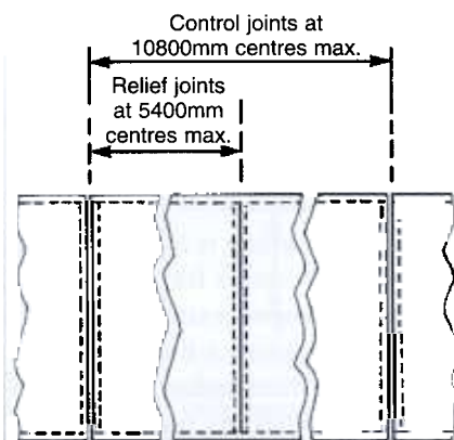
Fig. 20 RELIEF JOINT AND CONTROL JOINT SET-OUT
