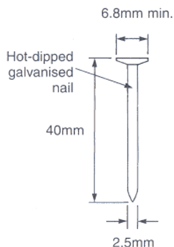
Fig. 28 HARDIFLEX® NAIL
