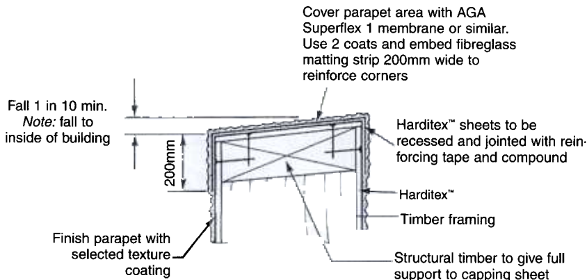
Fig. 68 PARAPET DETAIL
