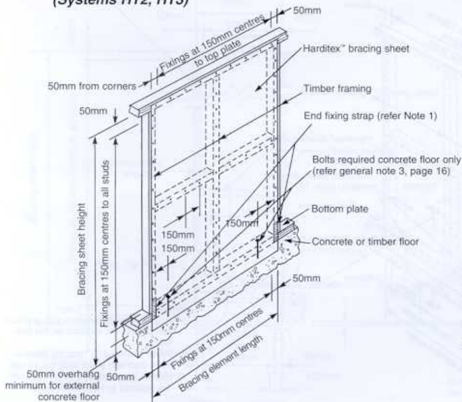
Fig. 39 HARDITEX™ ON TIMBER OR CONCRETE FLOORS WITH END STRAPS (Systems HT2, HT3)
