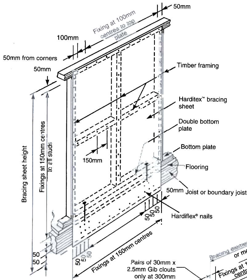
Fig. 51 HARDITEX™ / BRACELINE GROUP NAILING DETAIL TO TIMBER JOISTS (System HT11B)
