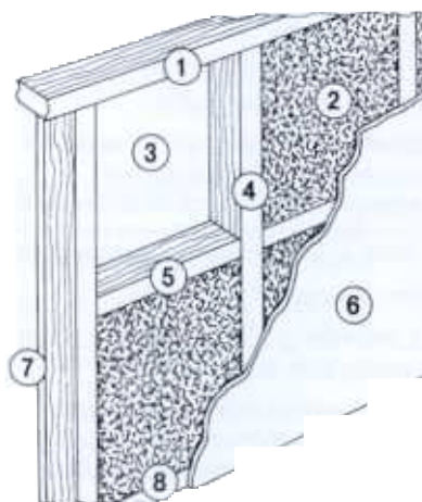
Fig. 35 TIMBER-FRAMED WALL WITH FIBREGLASS BATTS
