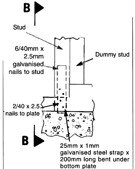
Fig. 48 END FIXING STRAP DETAIL FOR CONCRETE AND TIMBER FLOORS – 600MM-WIDE PANEL
