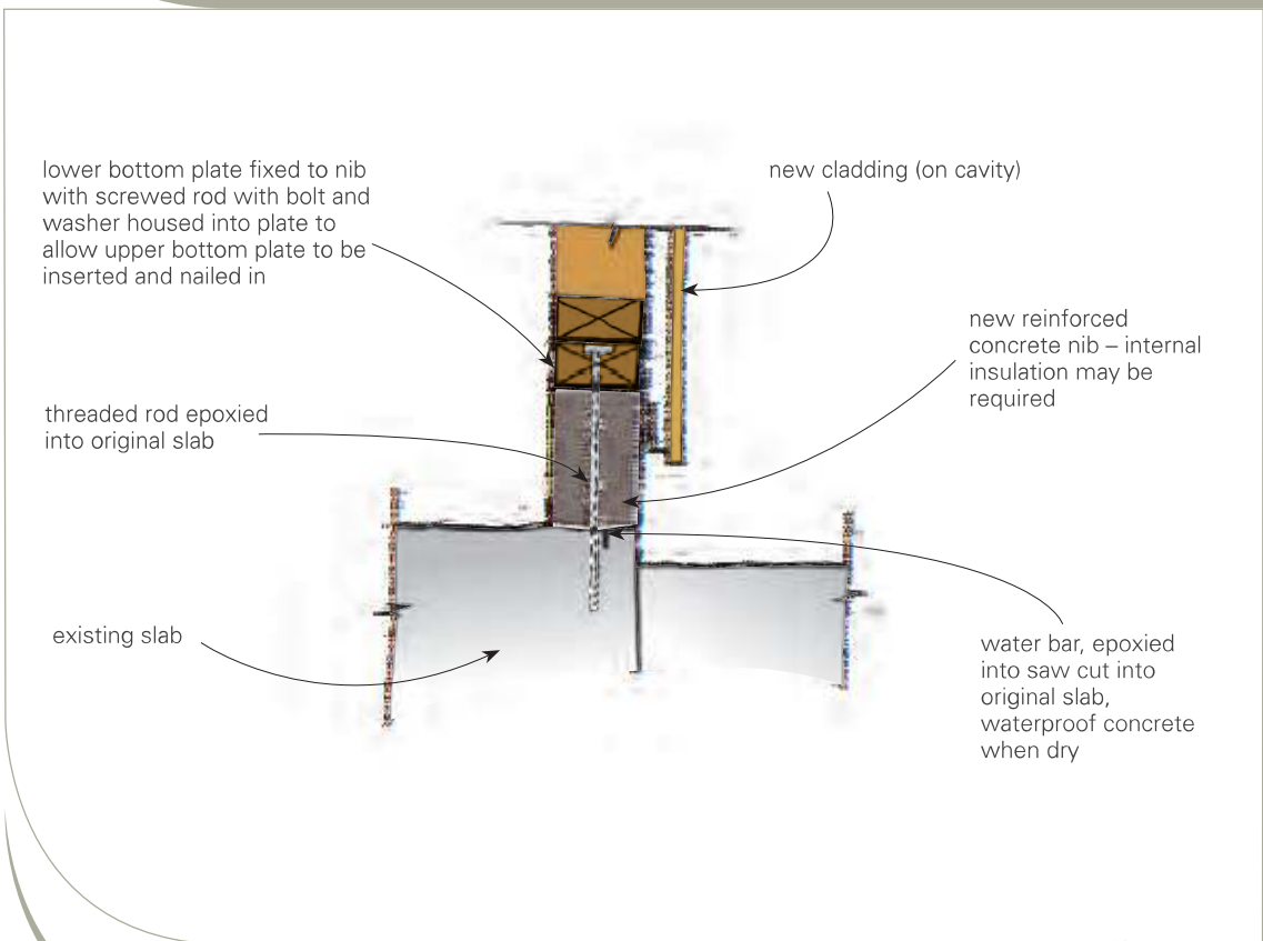
Figure 7.2 Nib detail with double bottom plate to lift base of wall.
